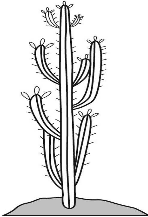
Diagram 4: A cactus plant
